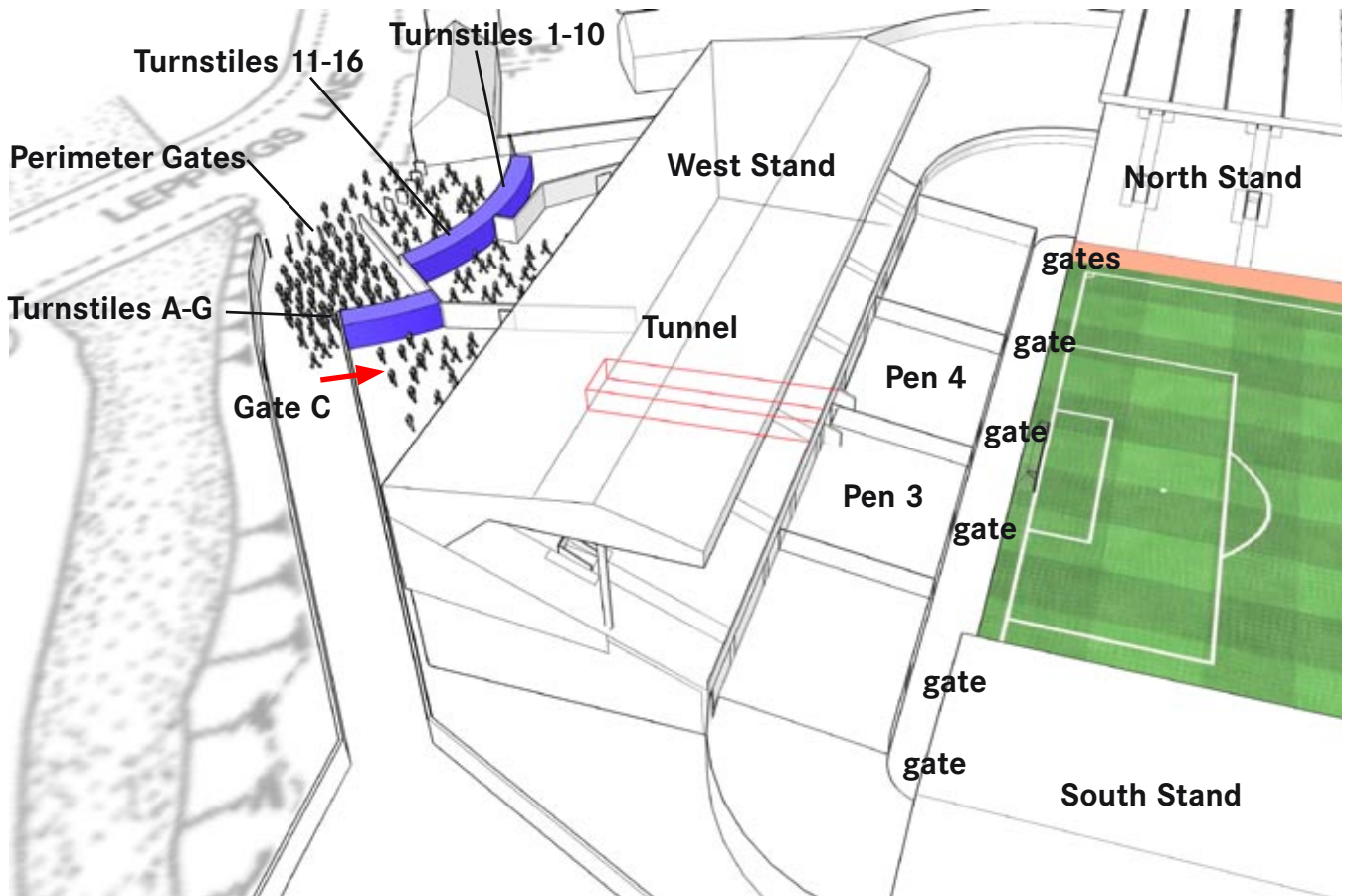
FIG 2. Detailed diagram showing the arrangement of turnstiles, gate C, the tunnel and pens in the West Stand (Leppings Lane Stand), Hillsborough, Sheffield.
